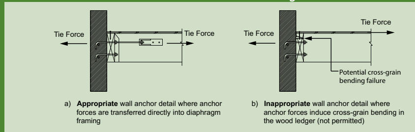
Figure C4.1.5B from SDPWS
